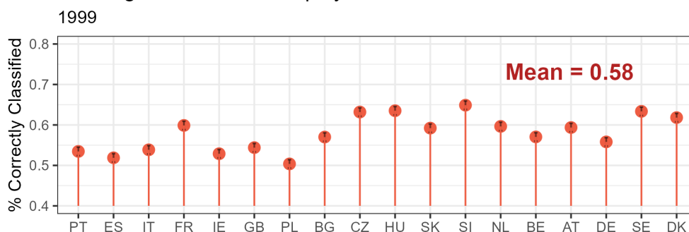
Figure F.1: Predictions with logistic regression.
