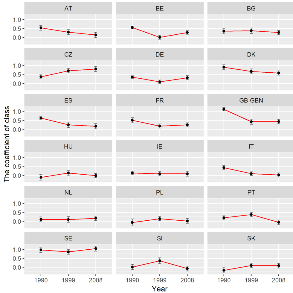
Figure G.2: Multilevel estimation.
