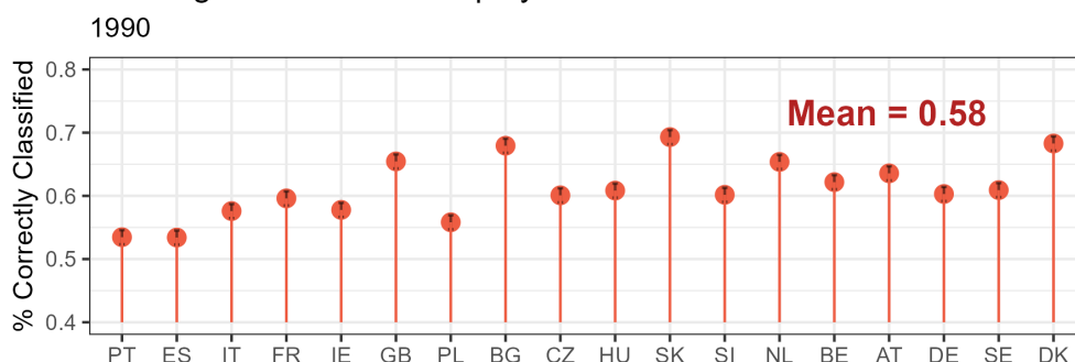
Figure 3: Predictions with logistic regression.
