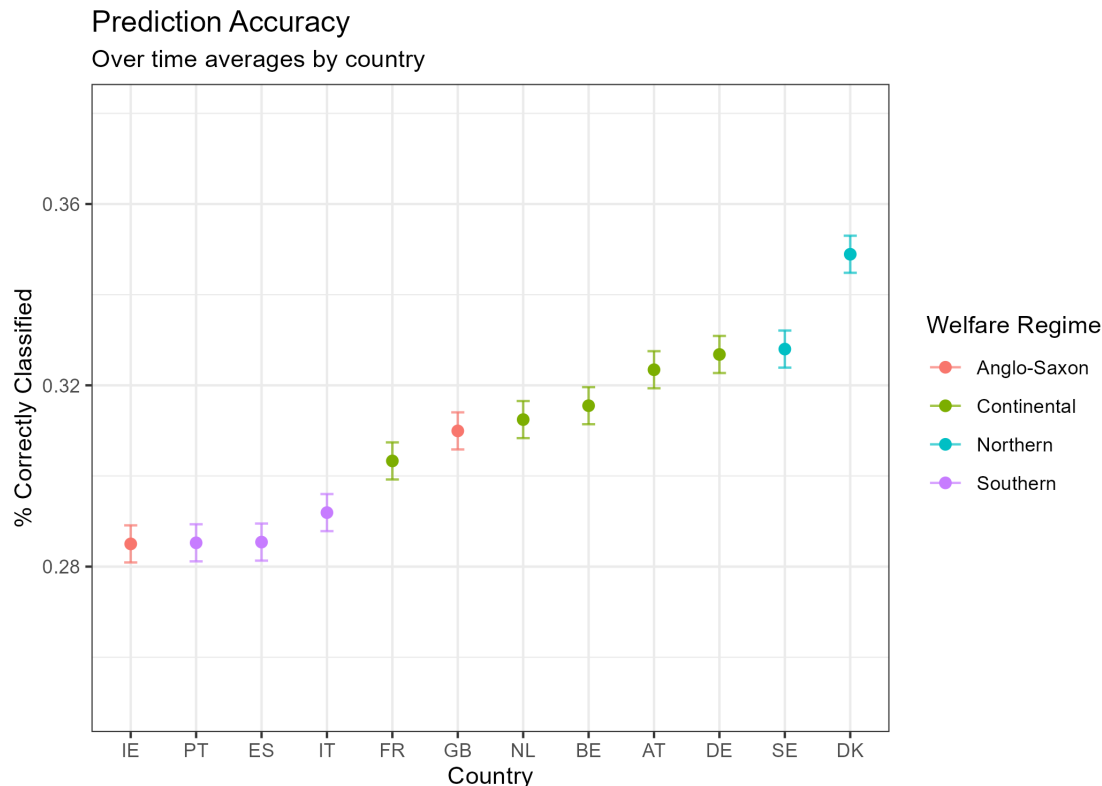
Figure 2: Predictions with multinomial logistic regressions.
