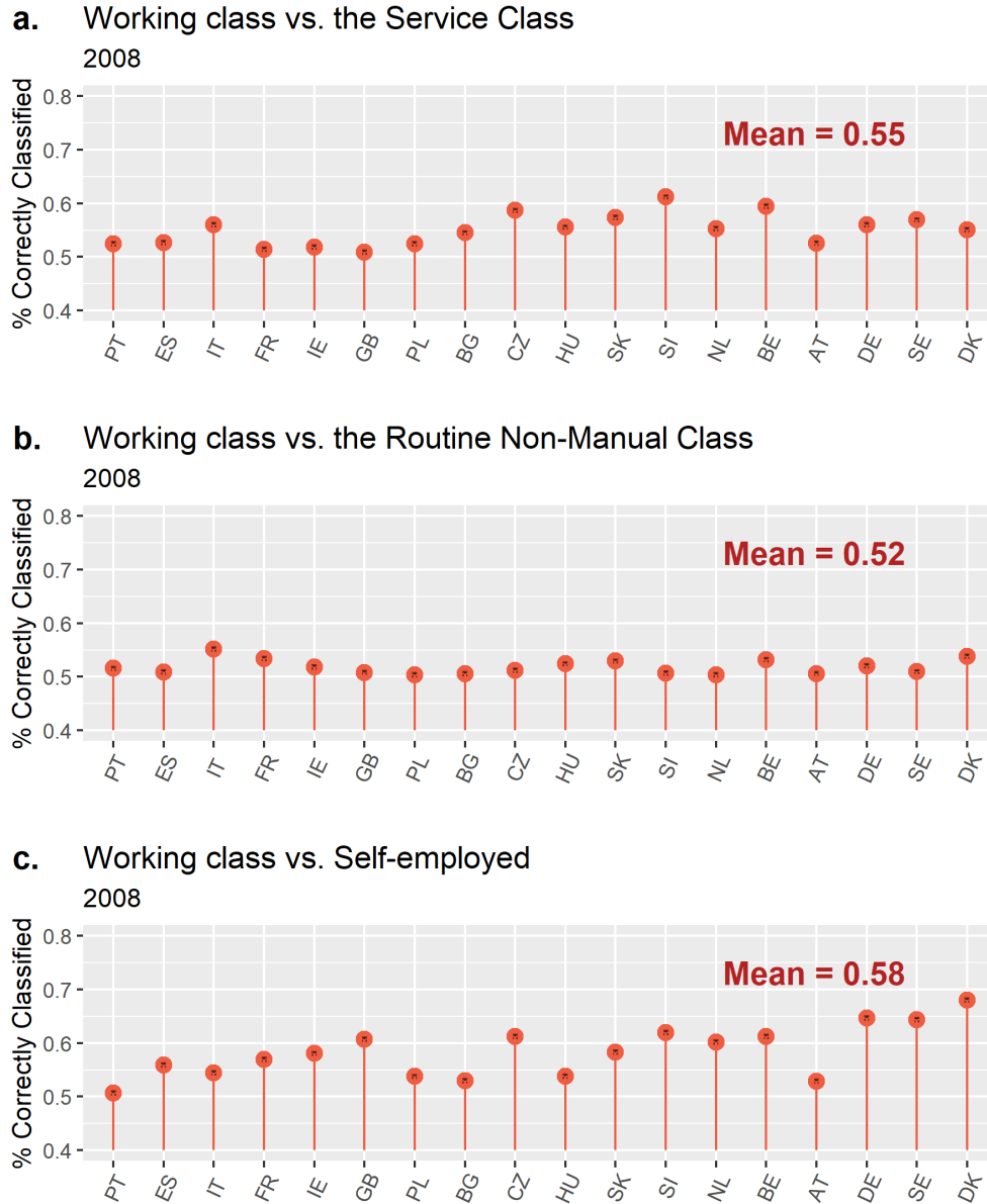
Figure F.2: Predictions with logistic regression.
