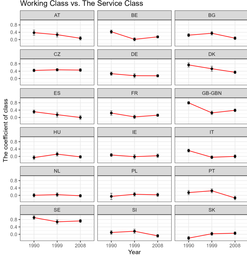
Figure 6: Multilevel estimation.
